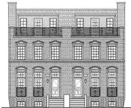
ELEVATION AND FLOOR PLAN
